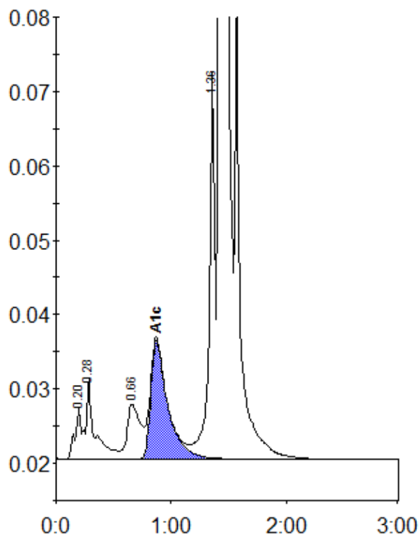
Peak table - ID: 10440506
